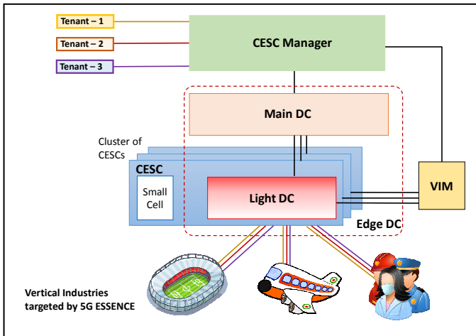
Fig. 5. The 5G ESSENCE high level architecture
