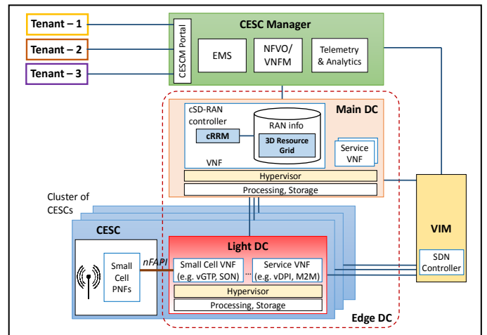
Fig. 4. The 5G ESSENCE architectural composition
